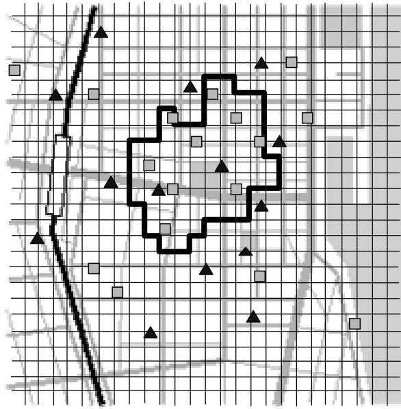
Figure 4: Optimal Region
