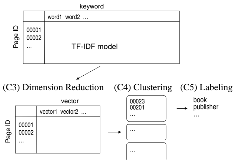
Figure 7: Concepts Extraction (2)
